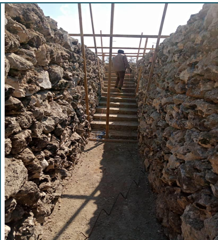
Construction of Cattle Dip in Simanjiro District
